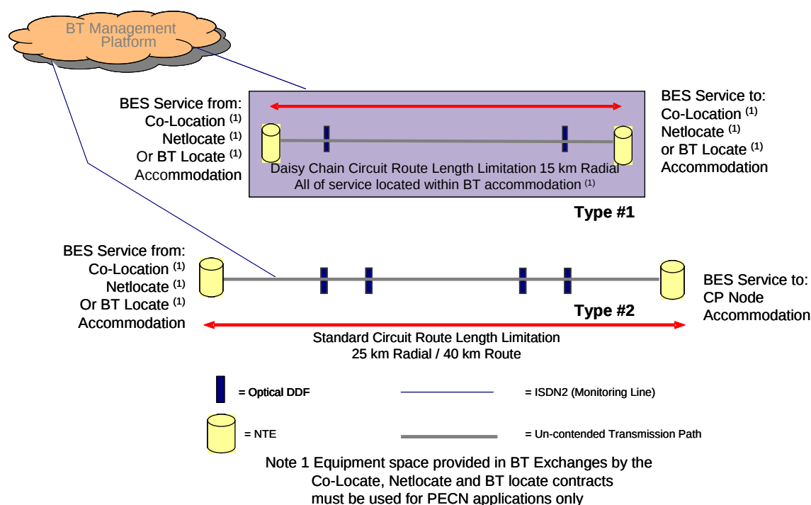
Figure 1. BES 155 Service Configuration
