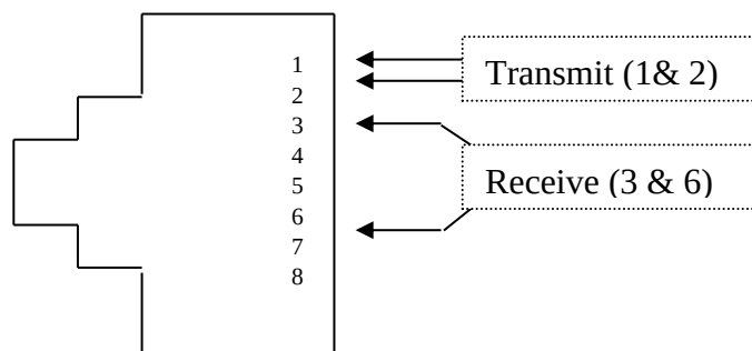
Figure 2. BES 100 NTE RJ45 Connector Pin Out Connections
